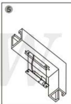
5 Mount lock body on the door frame and test
